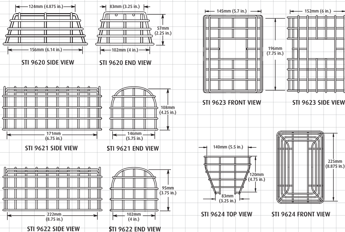
▼ Motion Detector Cages dimensions and technical information (STI 9620, STI 9621, STI 9622, STI 9623 & STI 9624)
